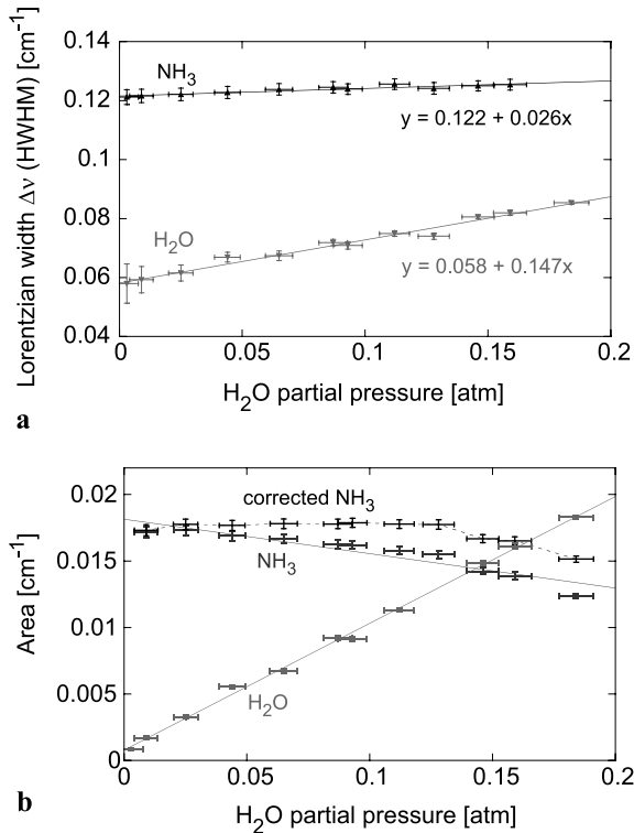
Fig. 7 Lorentzian width (a) and area (b) of the 6612.7 \text{ cm}^{-1} \text{NH}_3 and 6612.0 \text{ cm}^{-1} \text{H}_2\text{O} absorption features retrieved from the fits as a function of the \text{H}_2\text{O} partial pressure. Horizontal error bars represent the imprecision on the calculated \text{H}_2\text{O} partial pressure due to the incertitude in the relative humidity ( \pm 1.5\% RH) and temperature ( \pm 0.3^\circ\text{C} ) measured with the hygrometer; vertical error bars represent the imprecision (standard deviation) on the spectral parameters retrieved from the line fitting process. Straight lines correspond to a linear regression of the data, which provides the self- and \text{H}_2\text{O} -broadening coefficients
