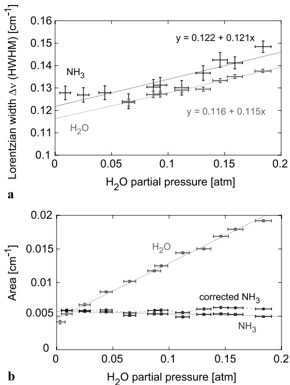
Fig. 9 Lorentzian width (a) and area (b) of the 6596.4 \text{ cm}^{-1} \text{NH}_3 and 6595.1 \text{ cm}^{-1} \text{H}_2\text{O} absorption features retrieved from the fits as a function of the \text{H}_2\text{O} partial pressure. Error bars represent the imprecision on the \text{H}_2\text{O} partial pressure and on the spectral parameters retrieved from the fitting process (see Fig. 7)
