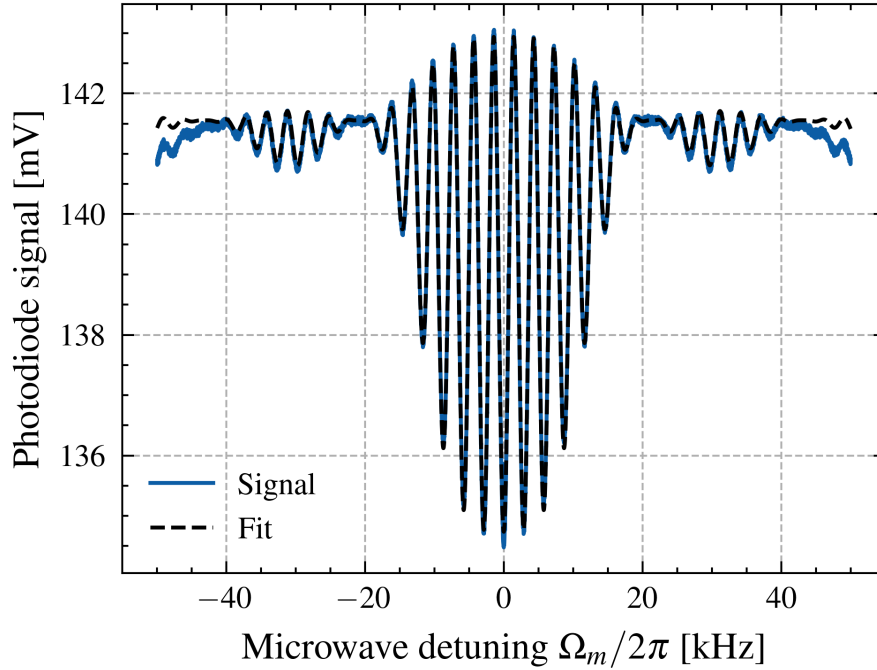
Figure 2.4: Example of Ramsey fringes acquired during the \mu\text{POP} measurement campaign.
