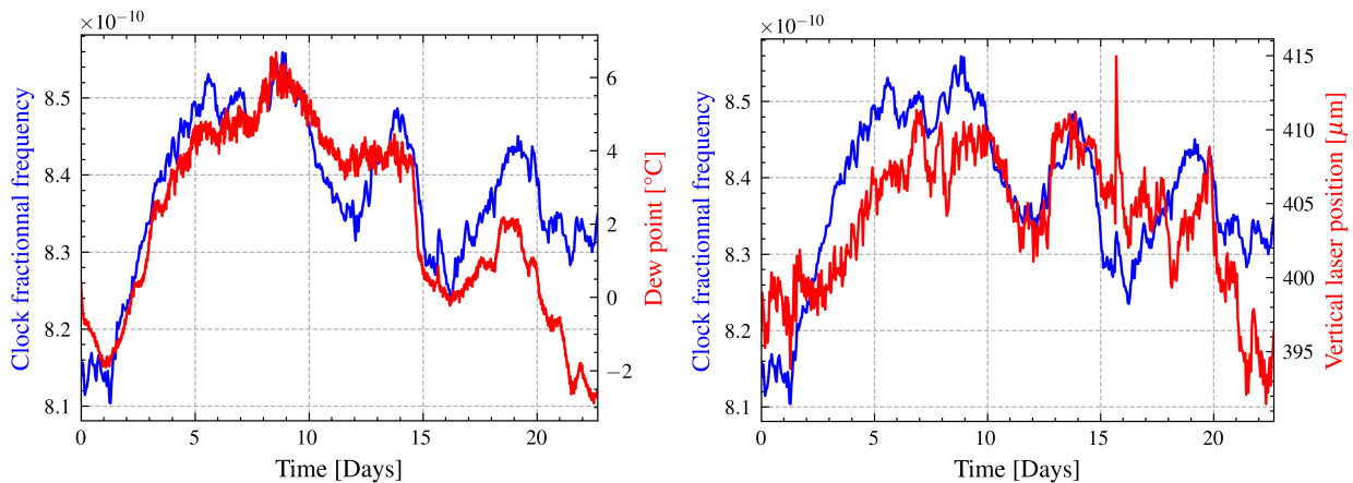
Figure 3.20: Left: (right) 96^\circ\text{C} clock fractional frequency with respect to the dew temperature (vertical laser position).
