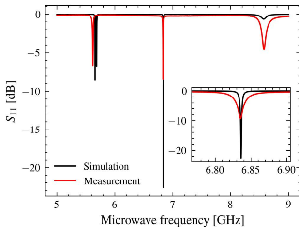
FIG. 7. Simulated and measured S_{11} spectrum of the cavity. The main figure and the inset share the same axis units.
