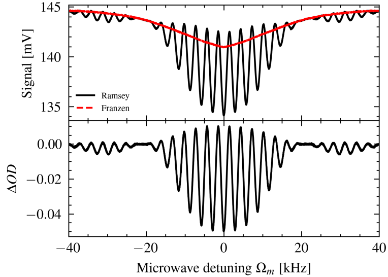
Figure 3.23: Top: Ramsey and Franzen signal with respect to microwave detuning. Ramsey and Franzen signals are taken sequentially for each detuning, starting at \Omega_m = 0 . In the absence of microwave (i.e. Franzen), the signal should be flat. The variation is solely due to the fluctuation of the light intensity. Bottom: Variation of optical density, independent of the light intensity fluctuations.
