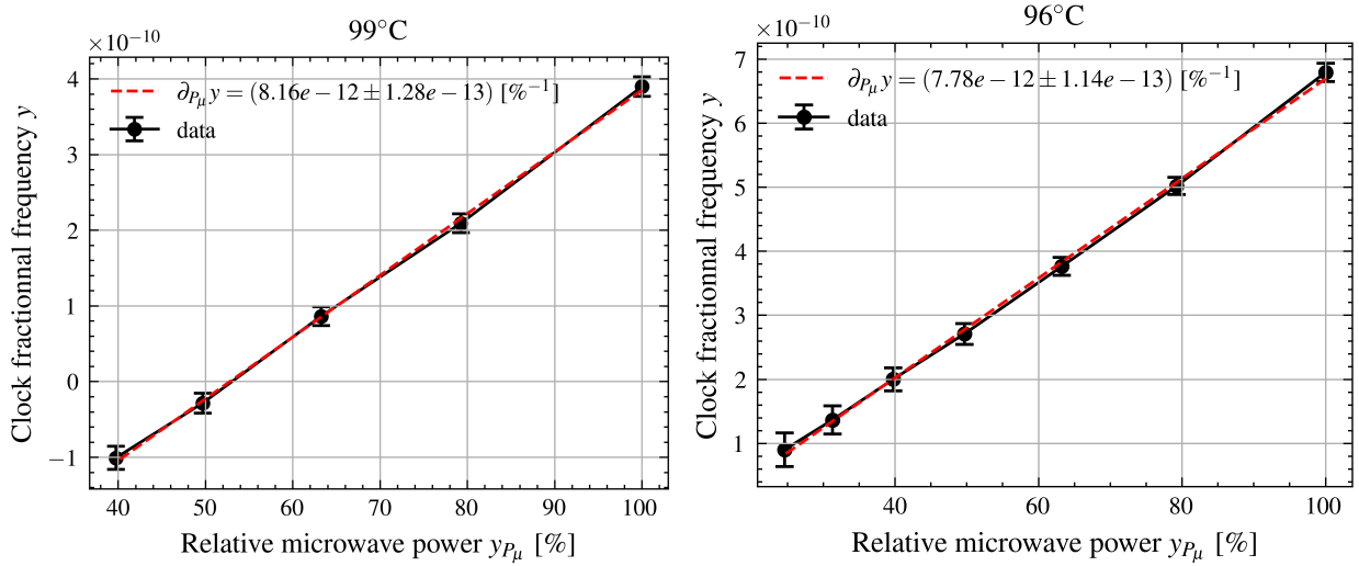
Figure 3.14: Left: (Right:) Clock fractional frequency with respect to microwave power for the 99°C (96°C) long-term measurement. The microwave powers are normalized by the nominal microwave power: 1.3 dBm.
